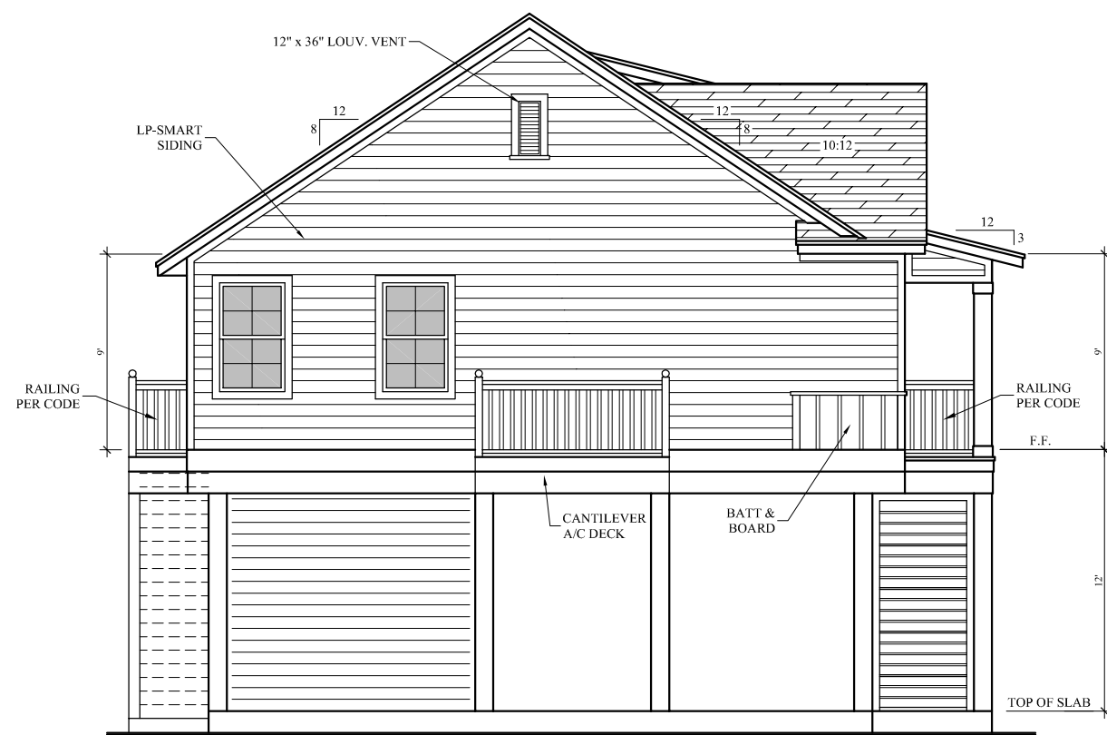
LEFT ELEVATION
